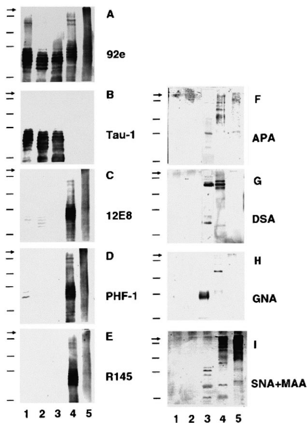
Fig. 1. Western and lectin blot analyses of various pools of tau. Isolated tau preparations (3.0 \mu\text{g}/\text{lane} ) were separated by 10% SDS-PAGE and the polypeptides were then transferred onto PVDF membranes. The blots were developed either with tau antibodies or with lectins. Lanes 1–5 are B-tau, N-tau, AD-tau, AD P-tau and PHF-tau, respectively. Antibody 92e (A) was used to detect the total amount of tau loaded in each lane. Several phosphorylation-dependent tau antibodies (B–E) were used to verify the phosphorylation state of tau. Various lectins (F–I) were employed to identify glycosylation and the specific sugar moieties. At the left side of each blot, the arrow indicates the top of the separating gel, and the short bars indicate the position of molecular mass markers (200, 98, 67 and 43 kDa, respectively).
